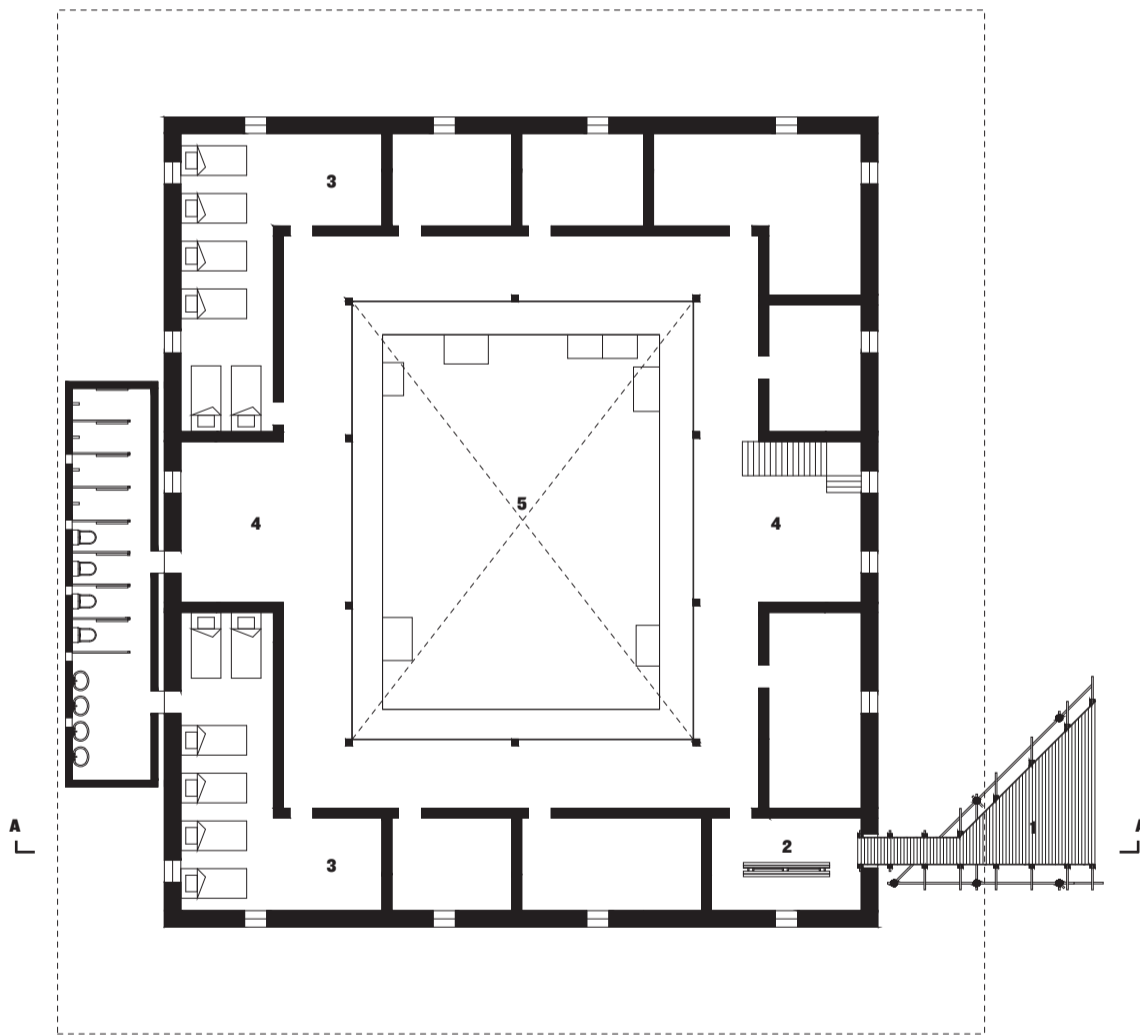
Plug-in first floor plan
