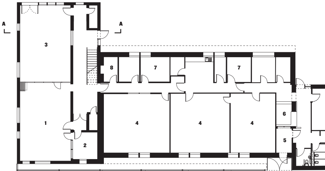
Swanlea 6th form ground floor plan
