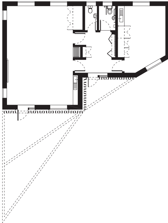
Seven Mills Primary floor plan
