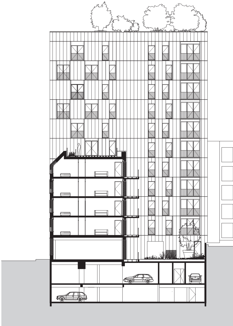
section AA
