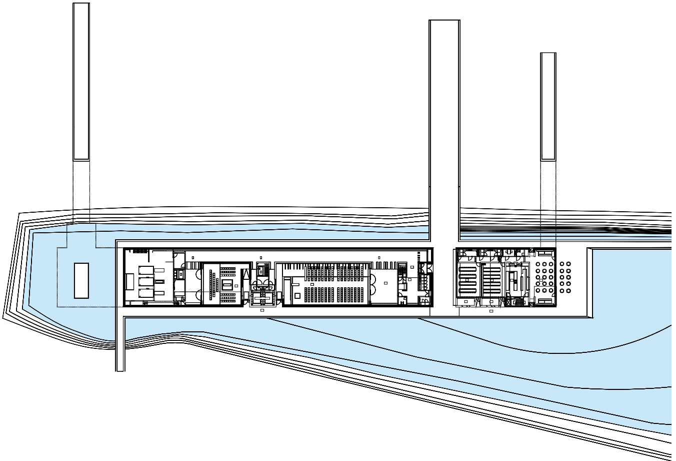
Hofheide Crematorium ground floor plan
