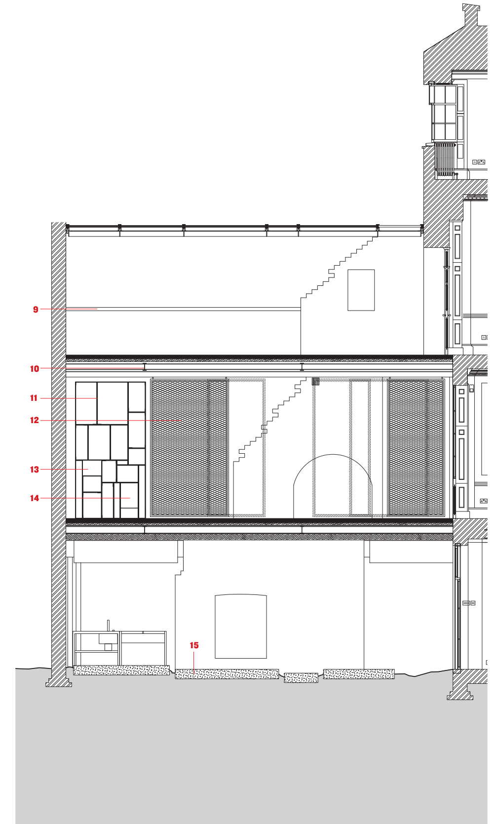
detail section AA
