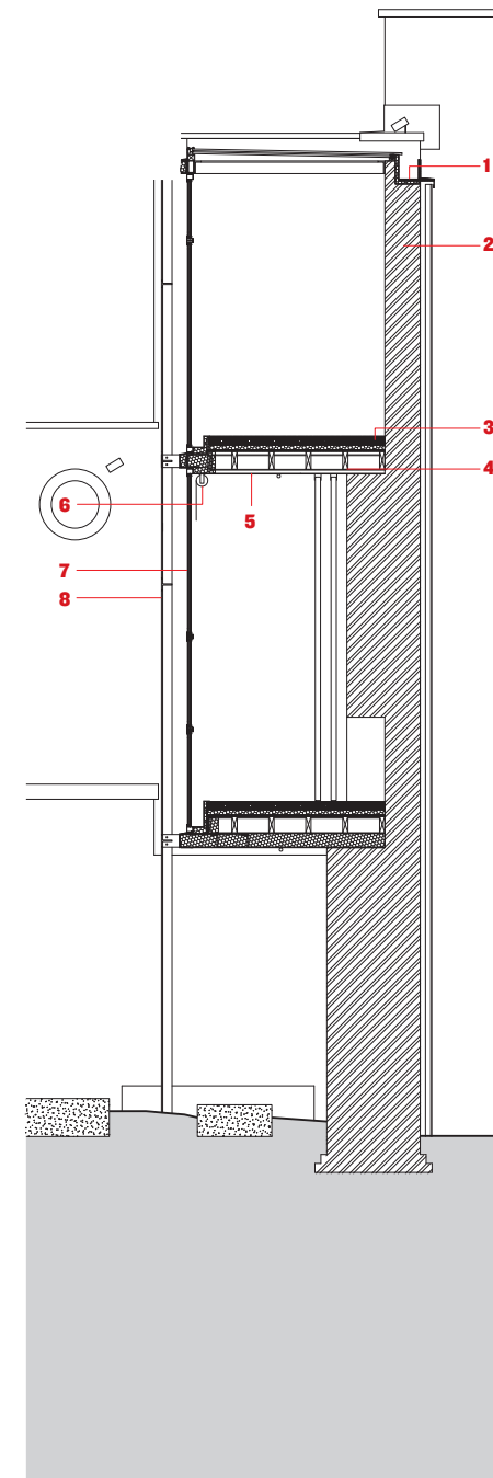
detail section BB
