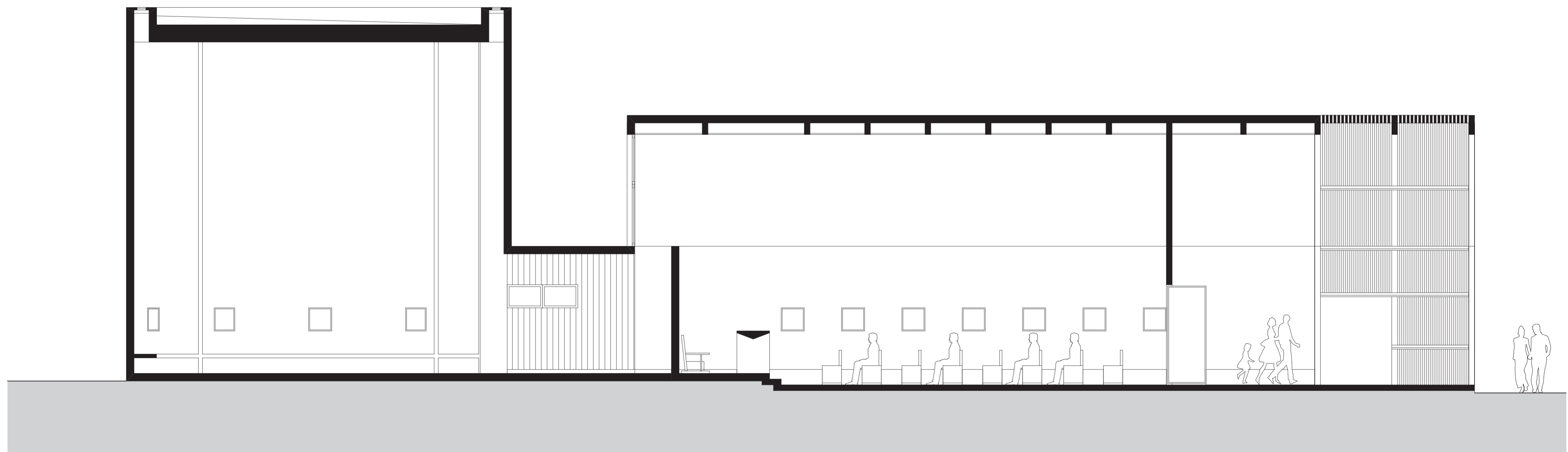
section BB
