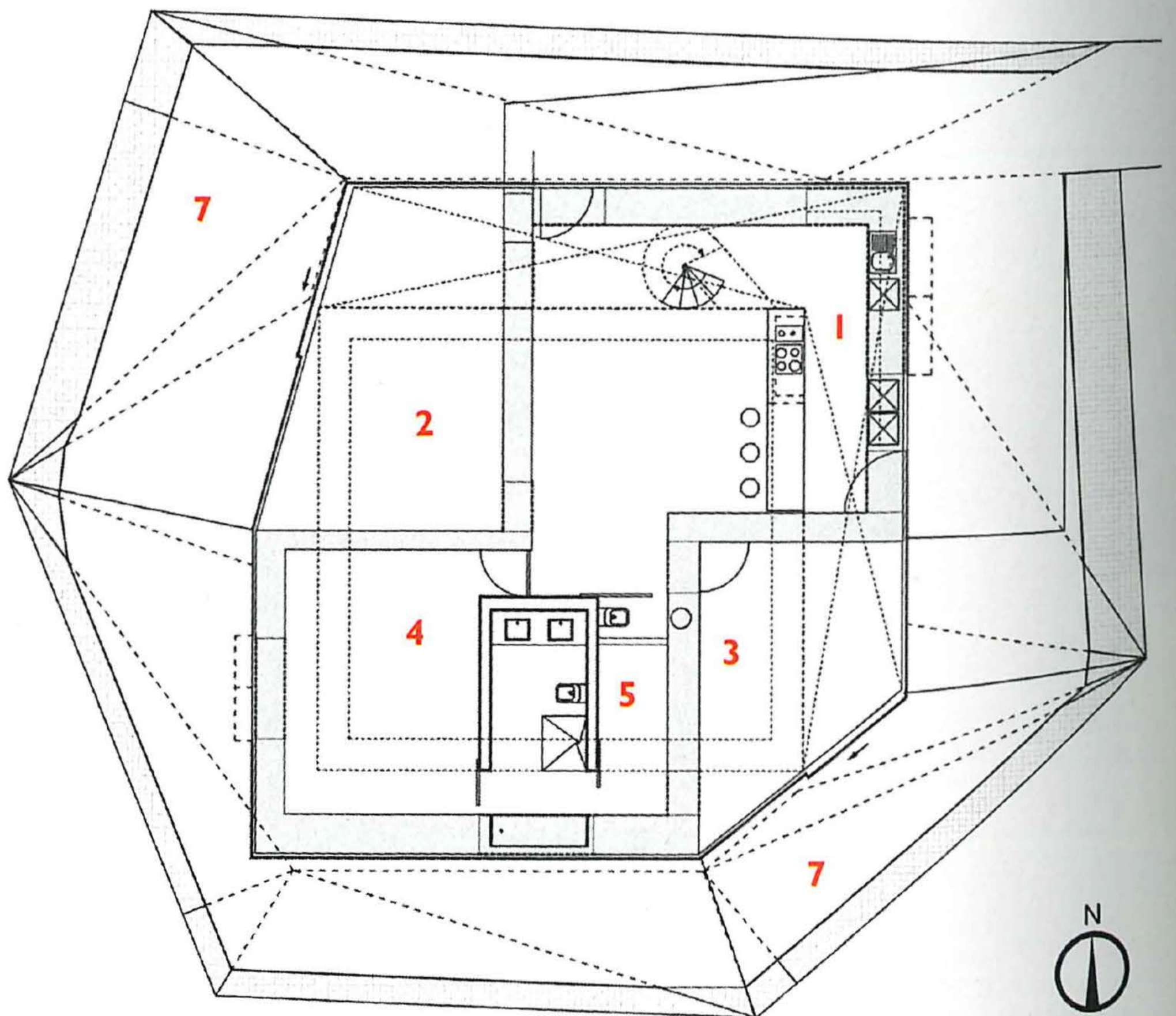
ground floor (scale approx 1:300)
