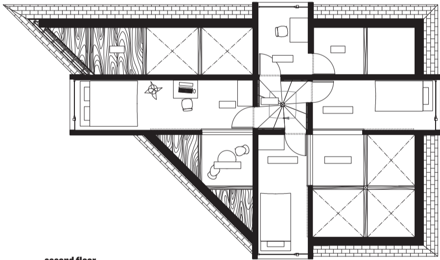
second floor
