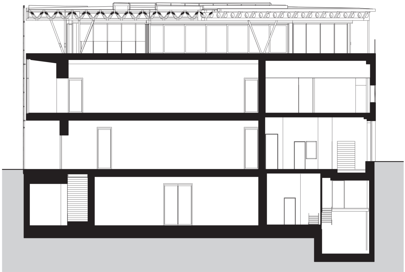
section BB
