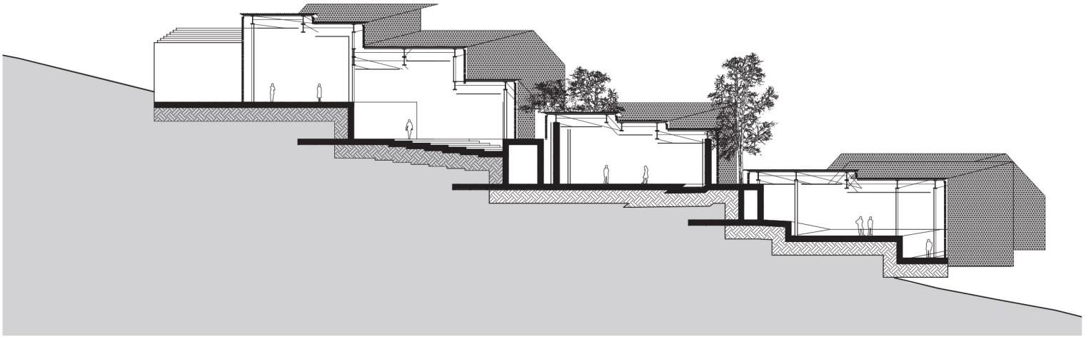
section BB
