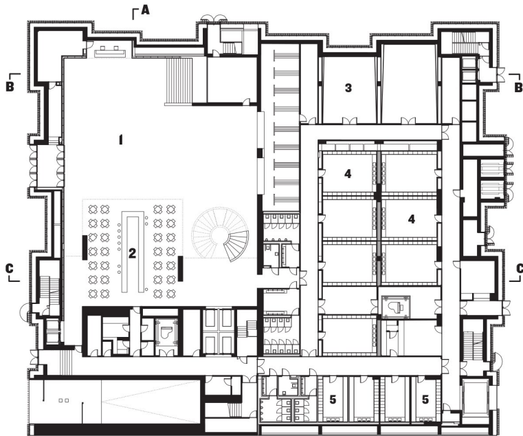
ground floor plan L A
