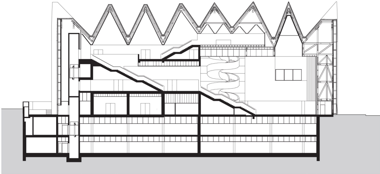
section BB
