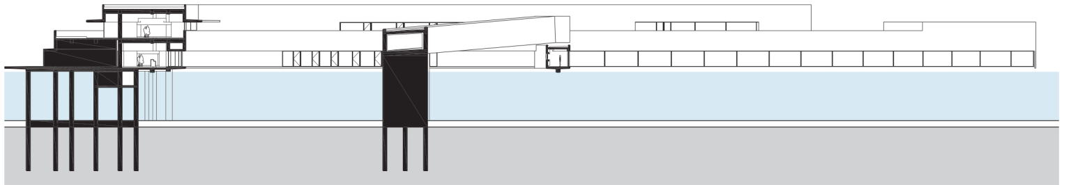
section BB
