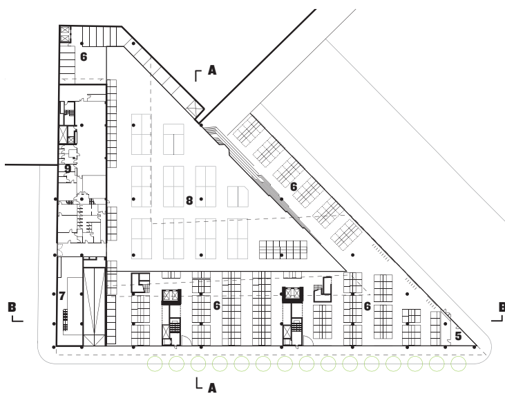
plaza level plan
