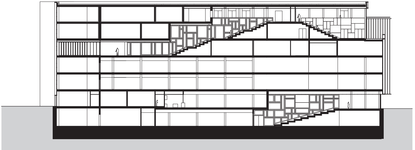
section BB
