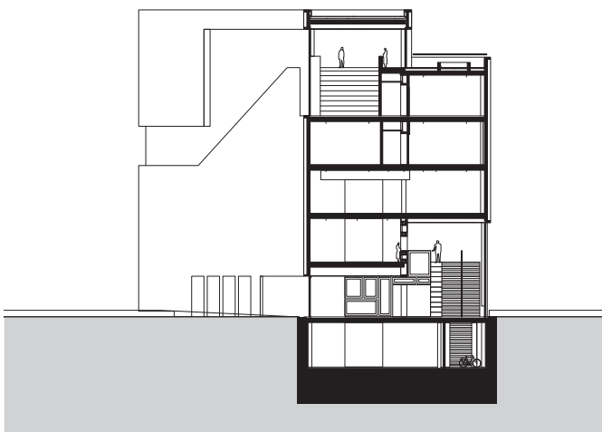
section CC
