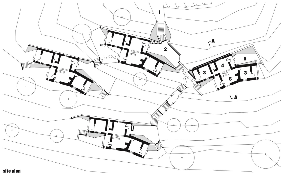
site plan
