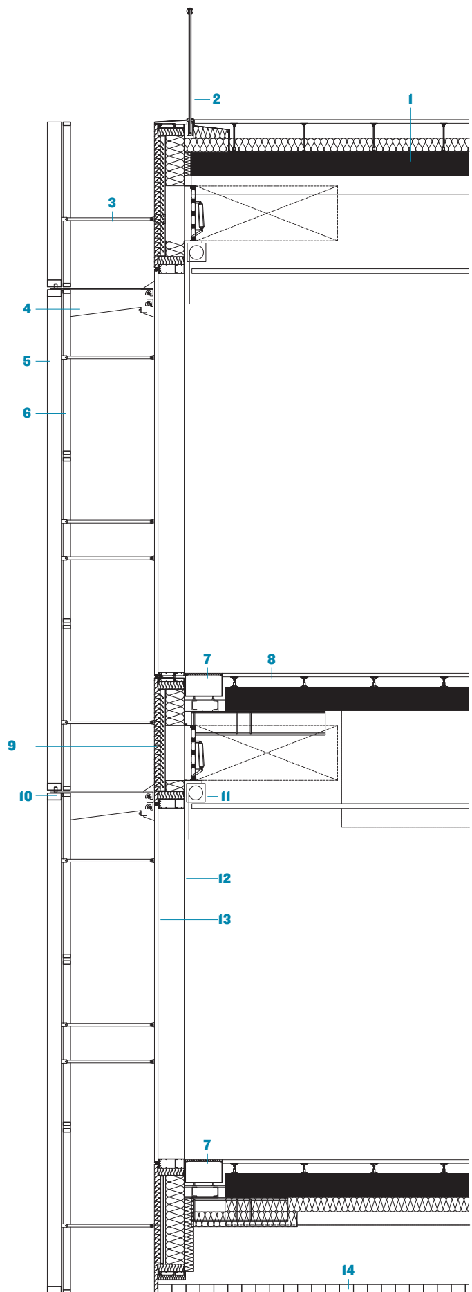
detail section through facade
