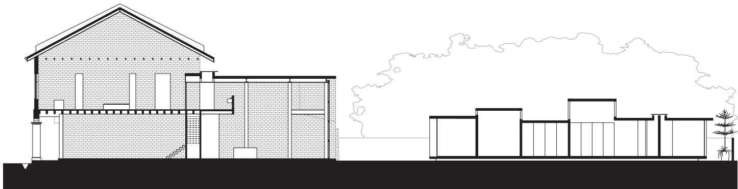
section AA through shophouse and guest house
