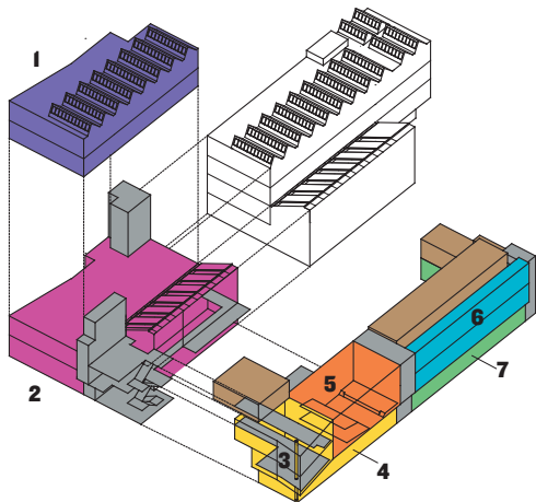
exploded axonometric
