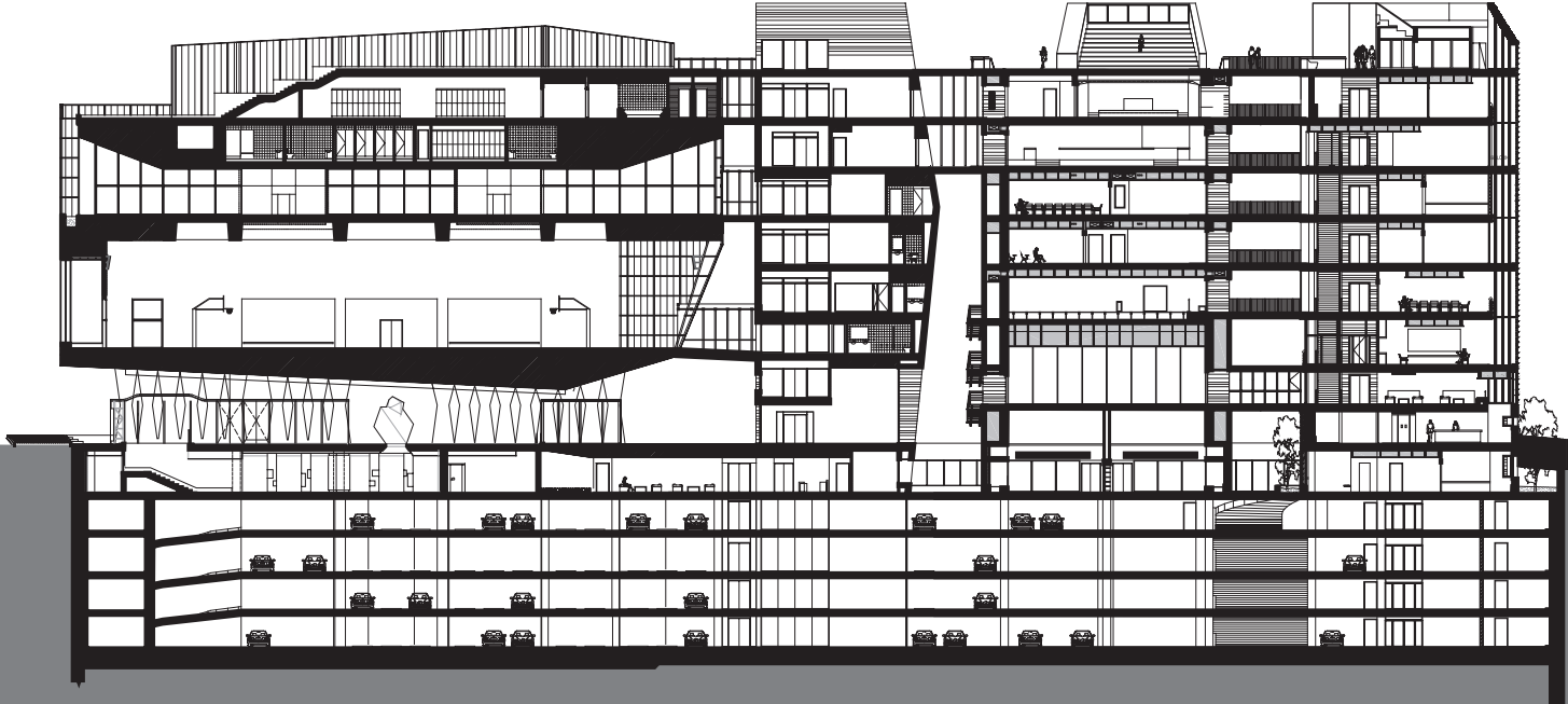
section AA
