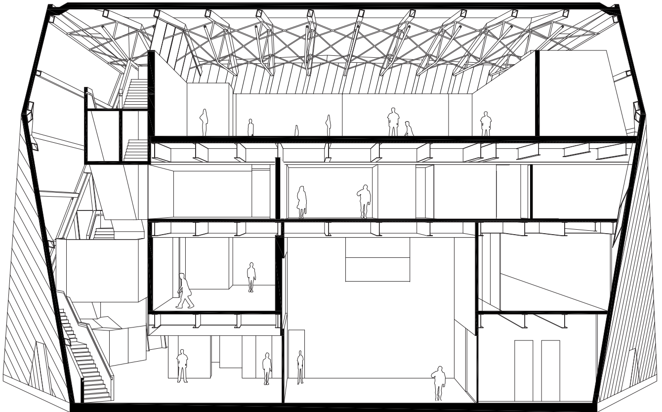
perspective section AA
