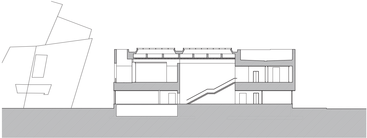
section BB
