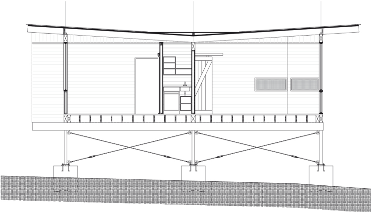
long section
