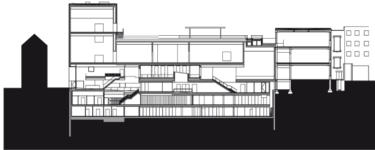
long section
