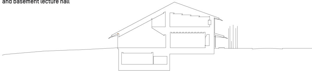
cross section through galleries and basement lecture hall
