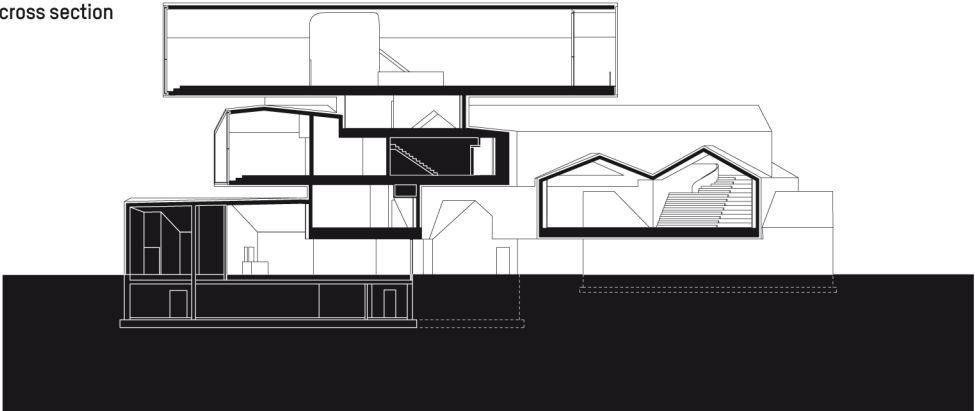
cross section
