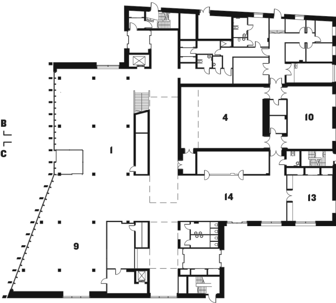
library ground floor plan
