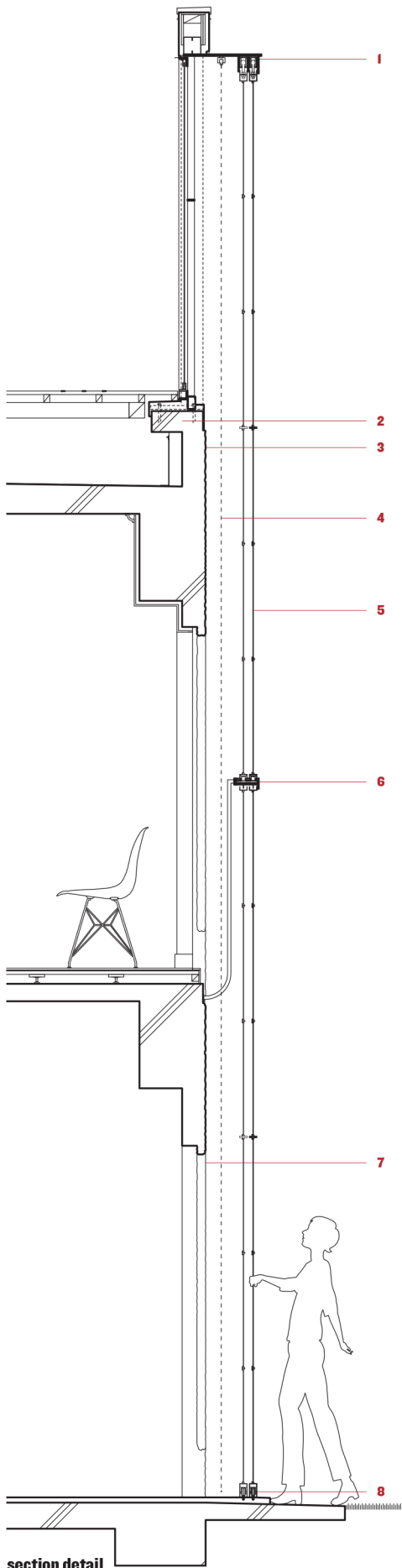
section detail
