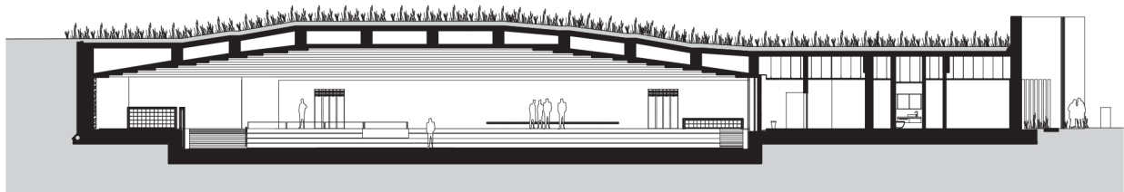
section BB
