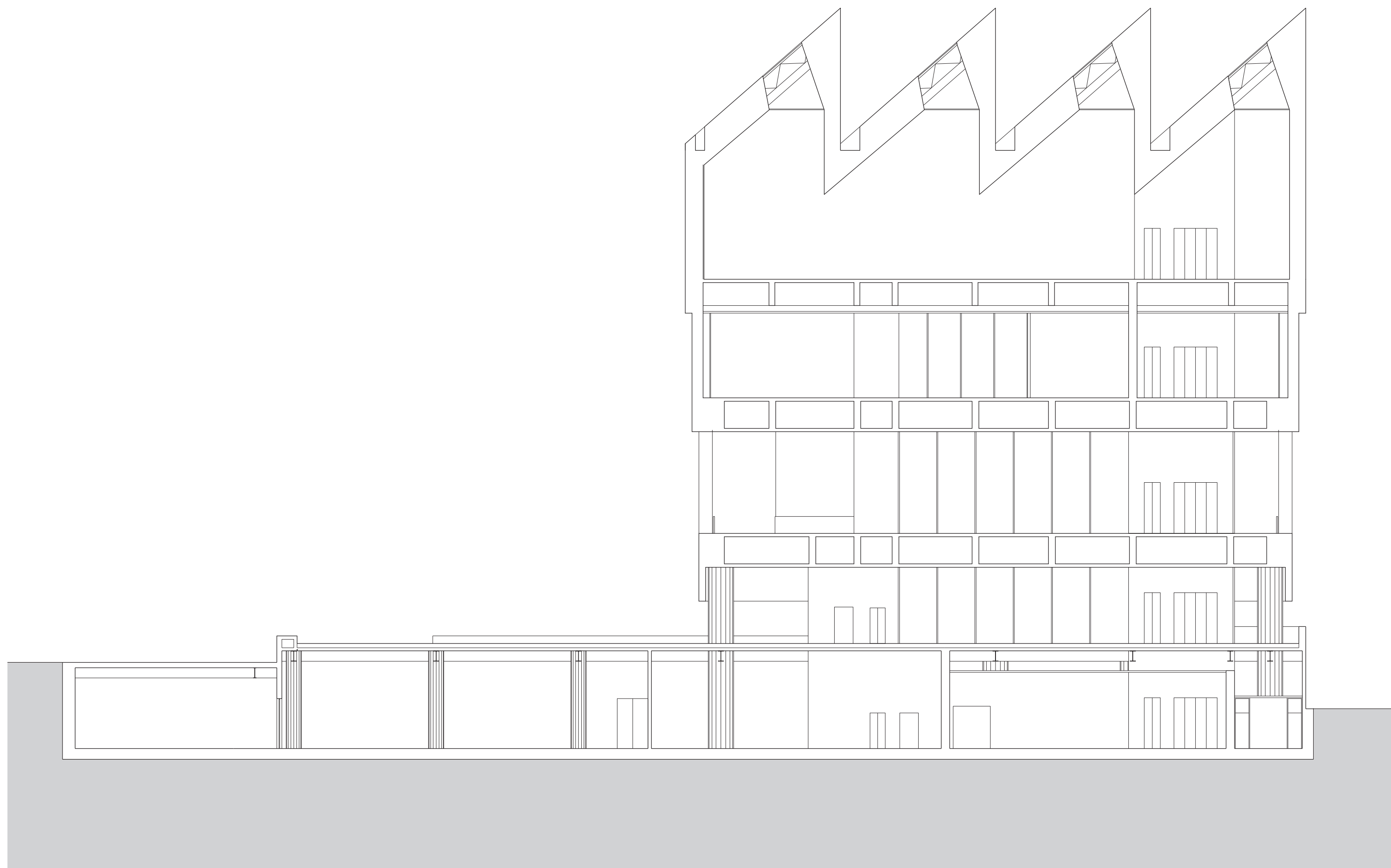
section bb
