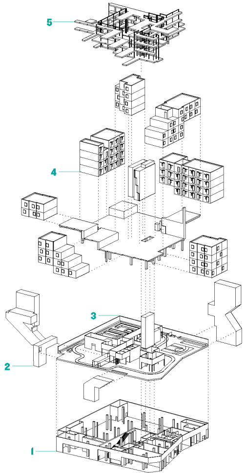
exploded projection
