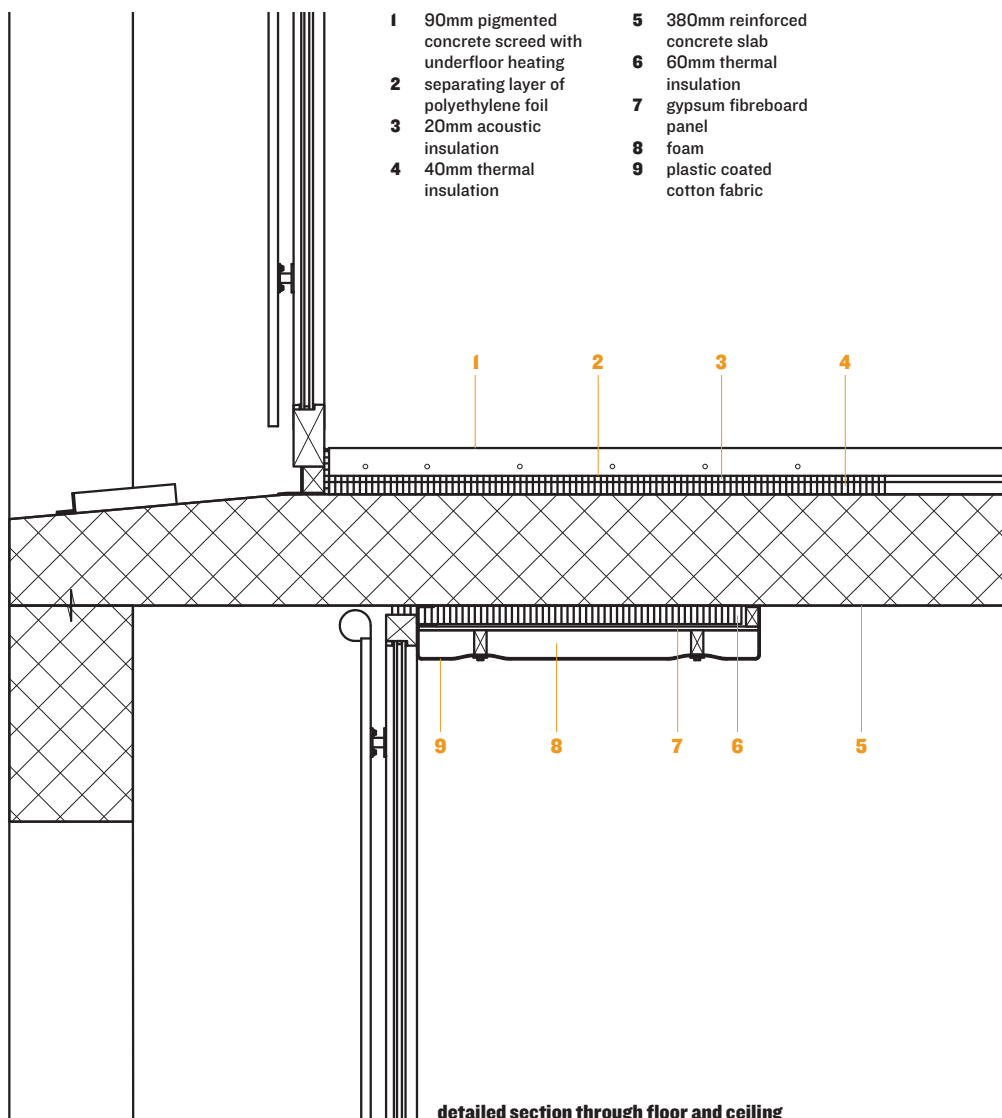
detailed section through floor and ceiling
