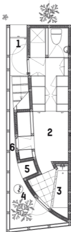
ground-floor plan
